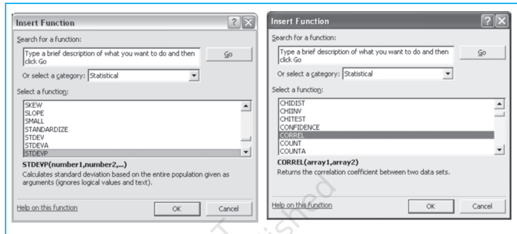
Fig. 4.7 : Function for Standard Deviation
